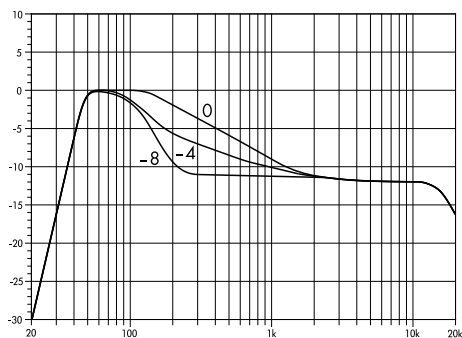
Frequency response correction of the CPL function for low and low-mid frequency level*
