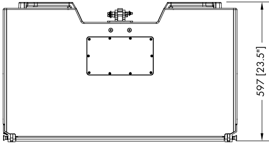
KSL8/KSL12 cabinet dimensions in mm [inch]
