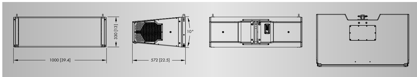
KSLi8 cabinet dimensions in mm [inch]
